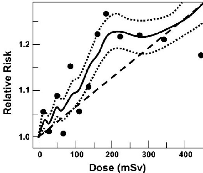
Figure 1. Estimated risks (relative to an unexposed individual) of solid cancer in atomic bomb survivors exposed to low radiation doses. Data points are placed at the mean of each dose category. The solid curve represents a weighted moving average of the points shown (dotted curves: \pm 1 SE), and the dashed straight line is a linear risk estimate computed from all the data in the dose range from 0 to 2,000 mSv. Age-specific cancer rates from 1958 to 1994 are used, averaged over follow-up and gender (Reproduced from Pierce & Preston, 2000 (21)).
